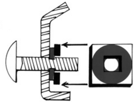
The 1/4" x 2" x 2" steel BOLT HOLE SUPPORT PATCH (with rubber bolt gripper under it) is welded on the inside of the rail giving it extra strength.
